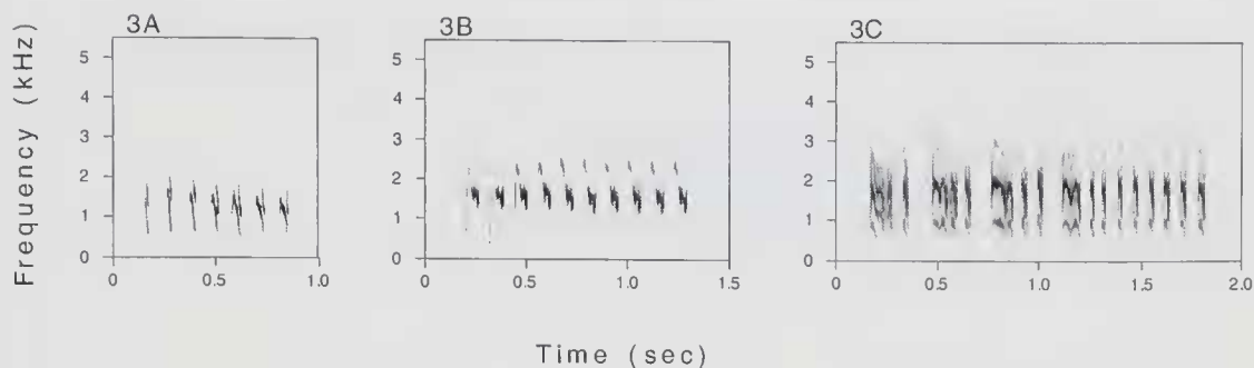
FIG. 3. Sonograms of "staccato whinny" vocalizations of Cercomacra antbirds: (A) "whinny" of Manu Antbird ( C. manu ) from Madre de Dios, Peru (K. J. Zimmer recording), (B) "whinny" of Mato Grosso Antbird ( C. melanaria ) from Mato Grosso, Brazil (R. Behrstock recording), and (C) song with "whinny" element of Bananal Antbird ( C. ferdinandi ) from Goias, Brazil (P. Donahue recording).
